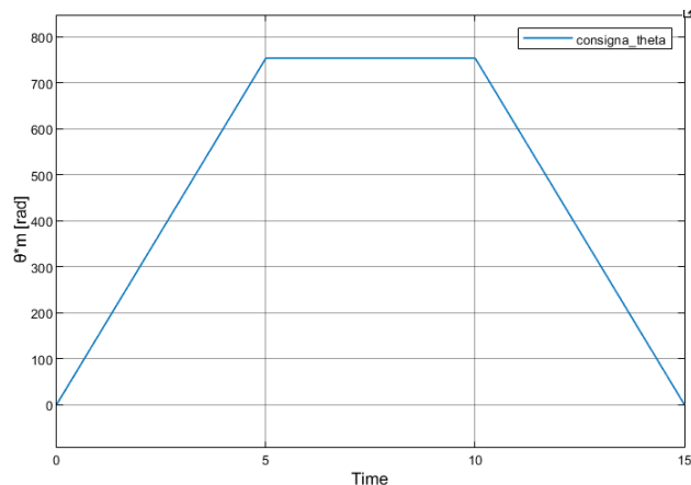
Figura 40: Consigna \theta_m^*
